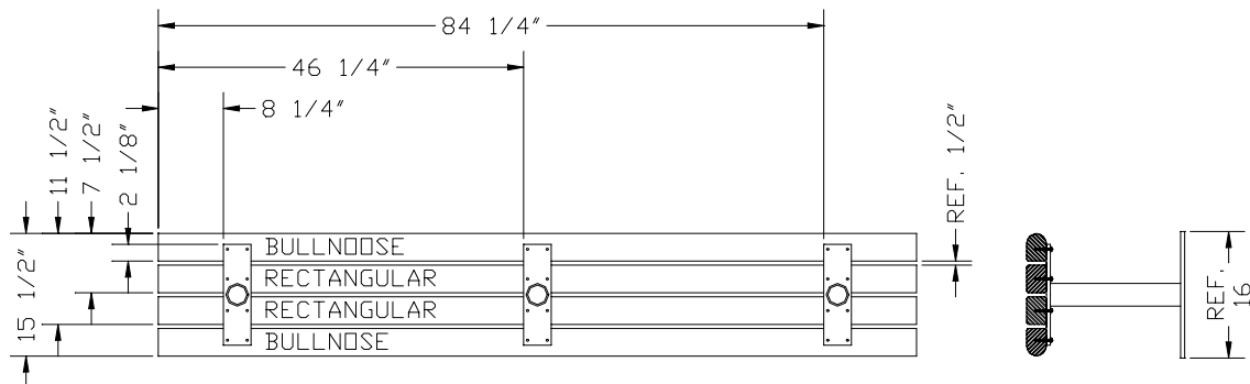
DIAGRAM 1: SEAT 8 FOOT LENGTH PORTABLE 210003 SHOWN
